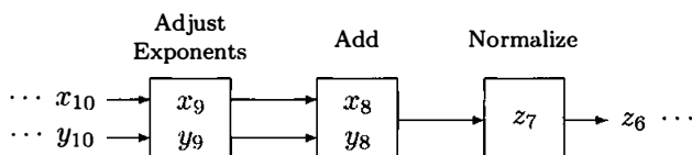
Figure 1.5.2. Pipelined addition
