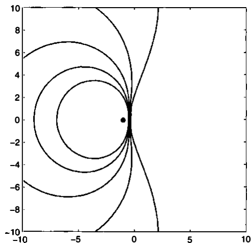
Figure 7.9.3. \Lambda_\epsilon(\text{Dem}_{50}(\beta)) with \beta^{49} = 10^8 and contours for \epsilon = 10^{-2}, \dots, 10^{-6}
