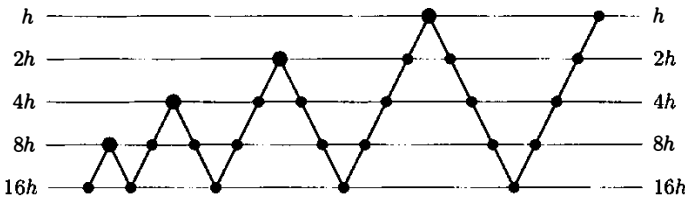
Figure 11.6.2. Full multigrid
