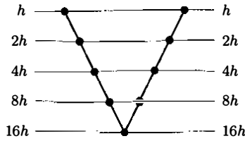
Figure 11.6.1. A V-cycle
