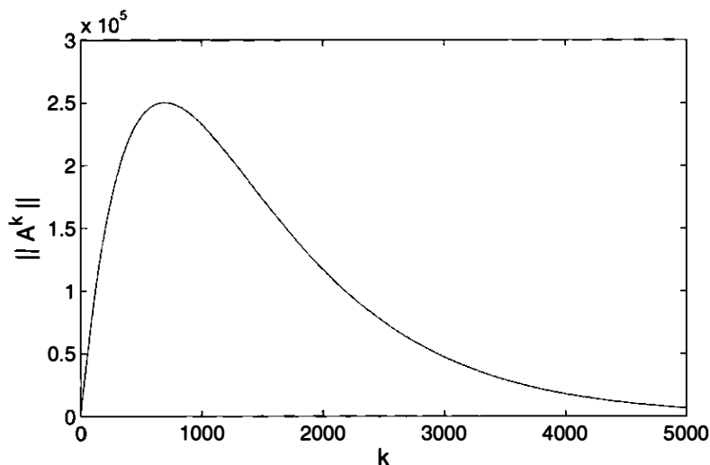
Figure 7.9.1. \|A^k\|_2 can grow even if \rho(A) < 1
